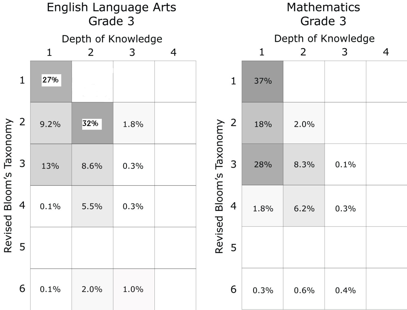
Figure 1: Density plots comparing the cognitive rigor of the English language arts and mathematics enacted curriculum (The Standards Company LLC 2008a, The Standards Company LLC 2008b).
